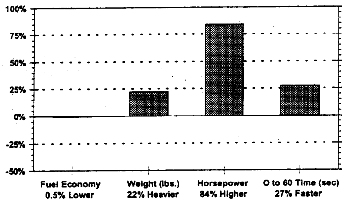
Percent Change from 1981 to 2001 in Average Vehicle Characteristics
