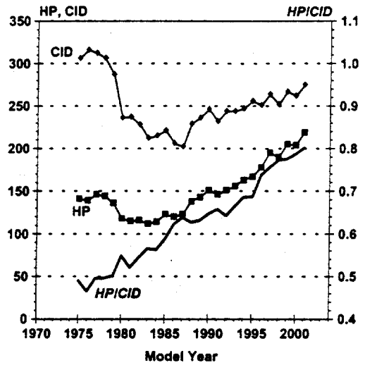
Pickup Horsepower, CID and Horsepower per CID
