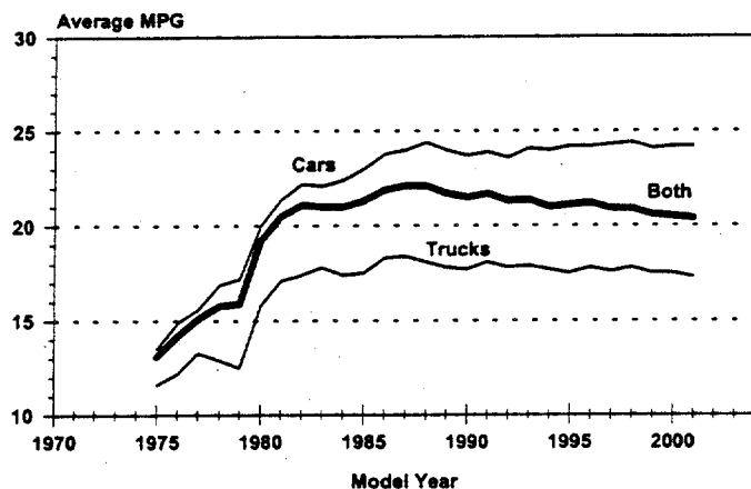
Fuel Economy by Model Year
