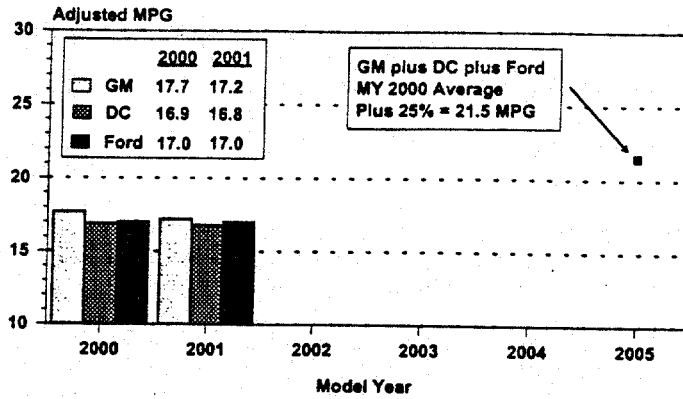
Light Truck Fuel Economy by Marketing Group
