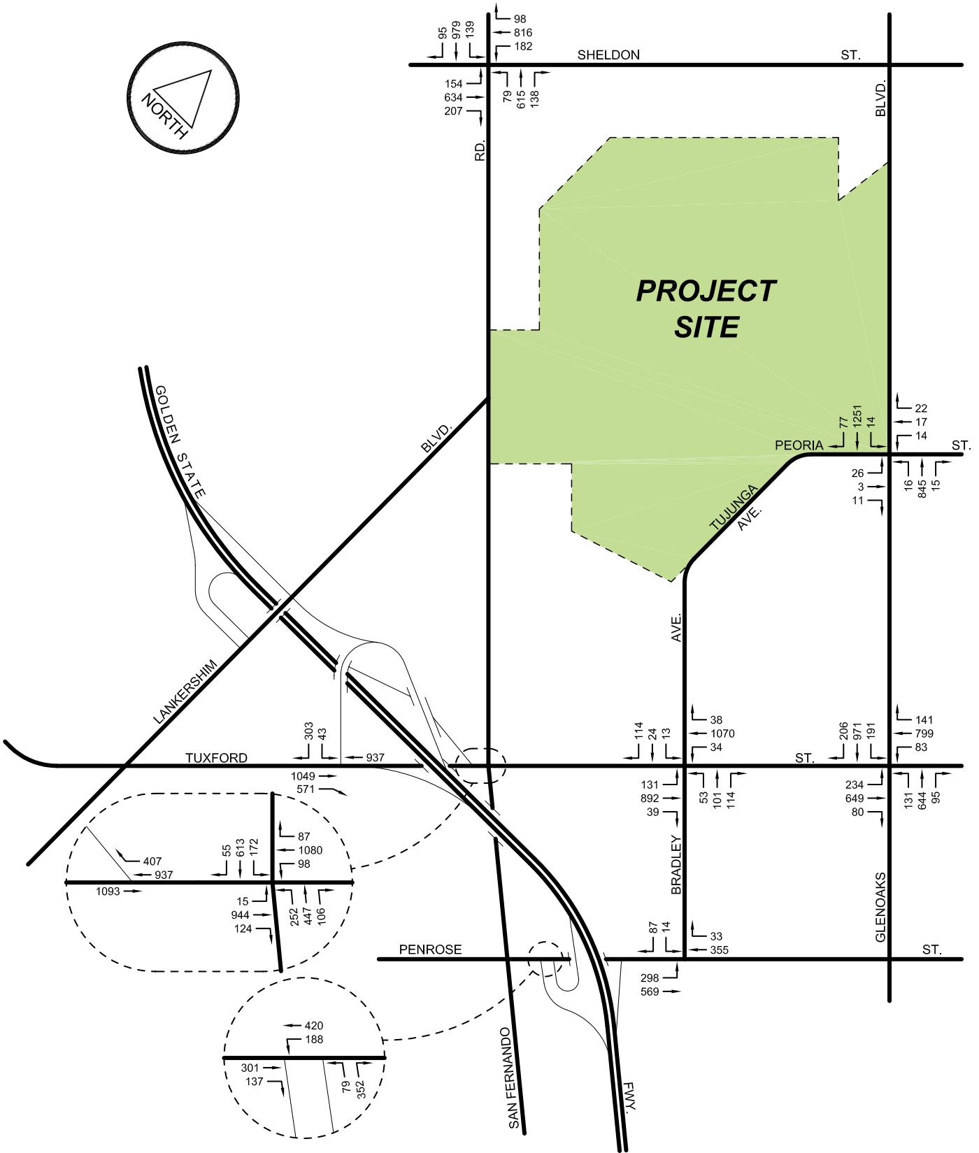
Figure 4.3-11 Future Without Project AM Peak Hour Traffic Volume (2012)
