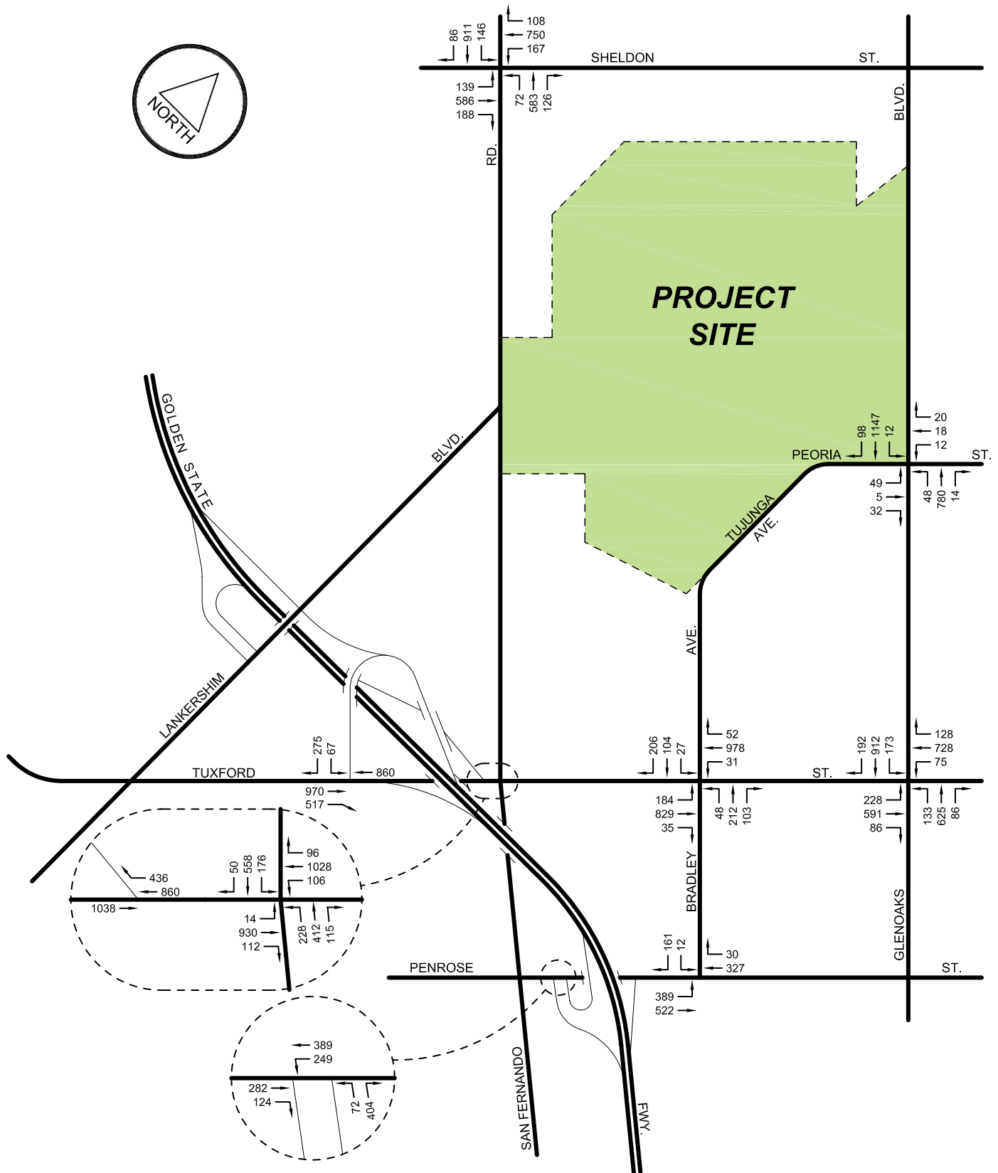
Figure 4.3-13 Future With Project AM Peak Hour Traffic Volumes (2007) Phase I Construction
