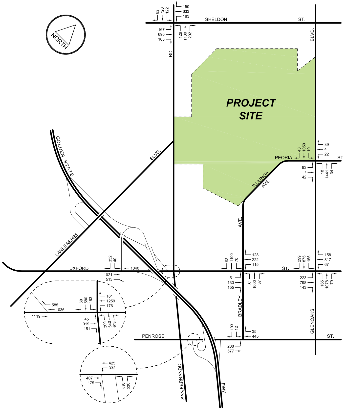
Figure 4.3-16 Future With Project PM Peak Hour Traffic Volumes (2008) Phase II Construction
