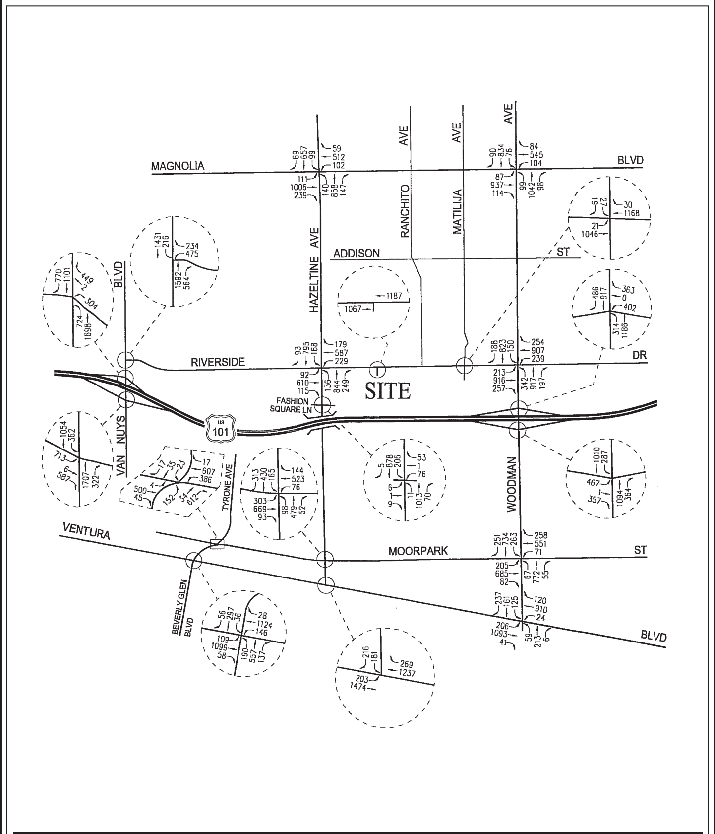
FIGURE 45 EXISTING TRAFFIC VOLUMES – WEEKDAY PM PEAK HOUR
