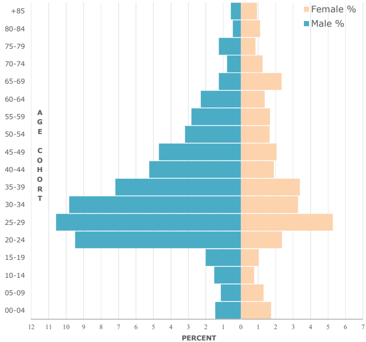
POPULATION PYRAMID
