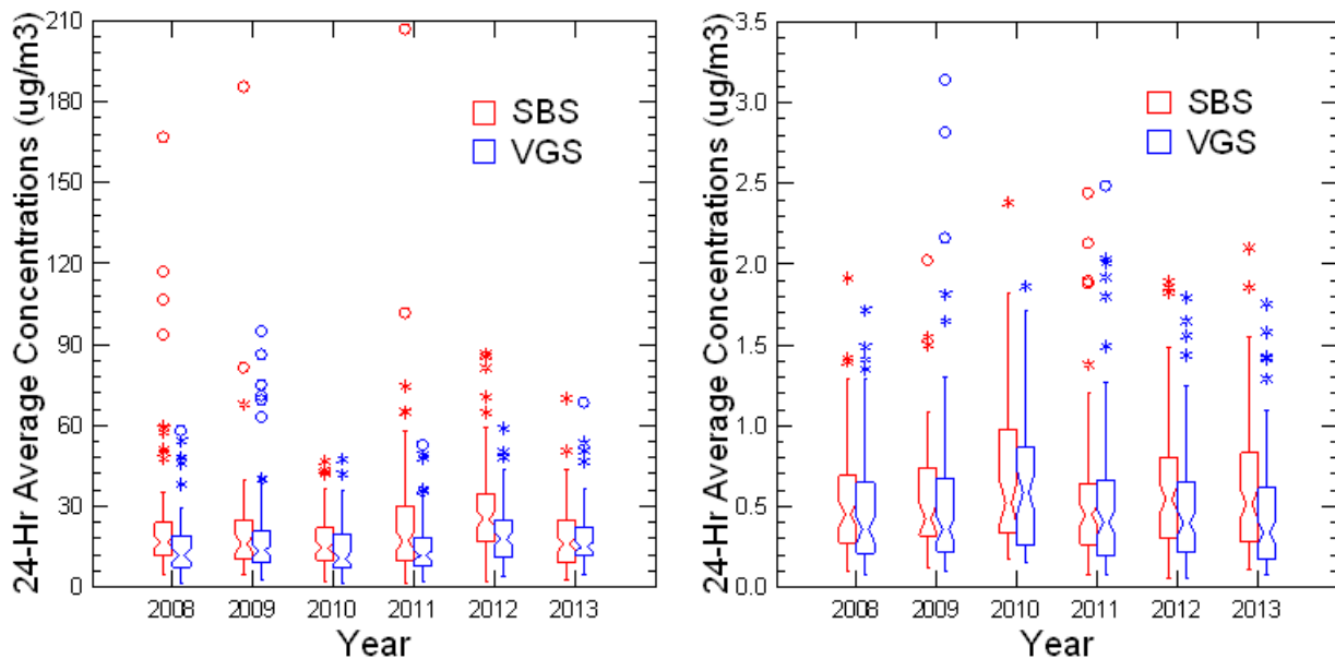
Figure 4-1. Notch box plot of daily 24-hr average concentrations during winter season at Sunshine Canyon Landfill (SBS) and Van Gogh (VGS) in years 2008 to 2013 for PM 10 (left) and BC (right).
